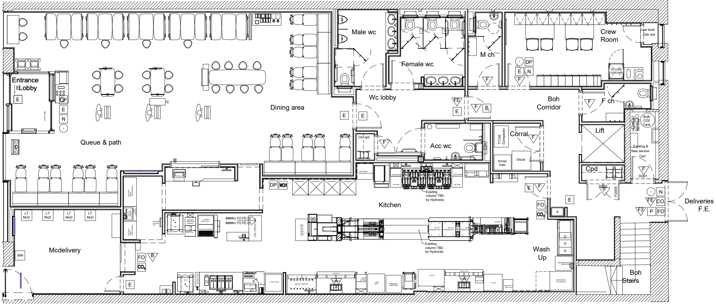
Ground floor
